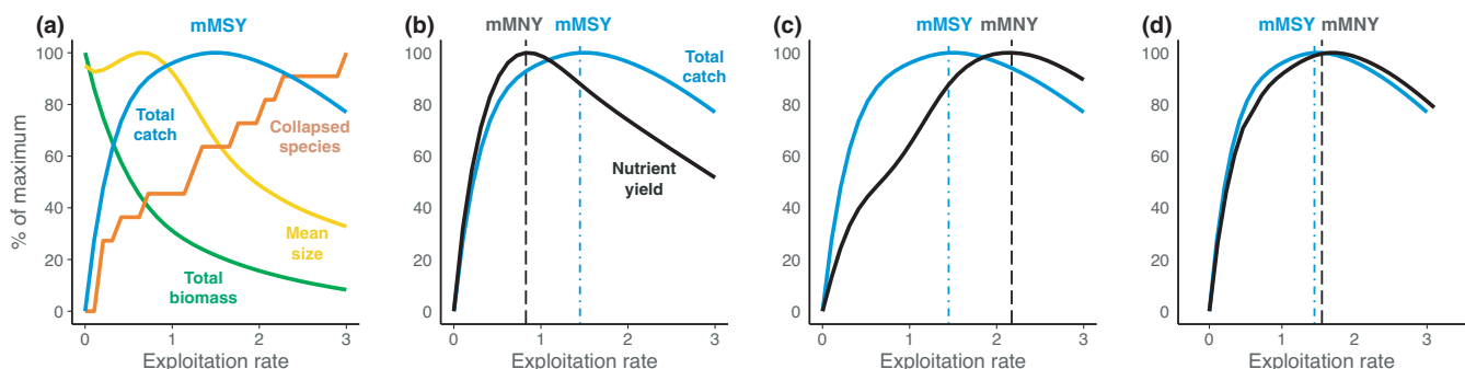
FIGURE 1 Theorised maximum nutrient yield curves for multispecies fisheries. (a) shows the effect of exploitation rate on total catch (blue), fishable biomass (green), mean size (yellow) and number of collapsed stocks (orange). Nutrient yield curves may be maximised at fishing levels (b) below mMSY (nutrient overfishing), (c) above mMSY (nutrient underfishing) or (d) similar to mMSY. Catch curves were generated using a generic size-based fisheries model of 15 interacting species with varying nutrient concentrations
