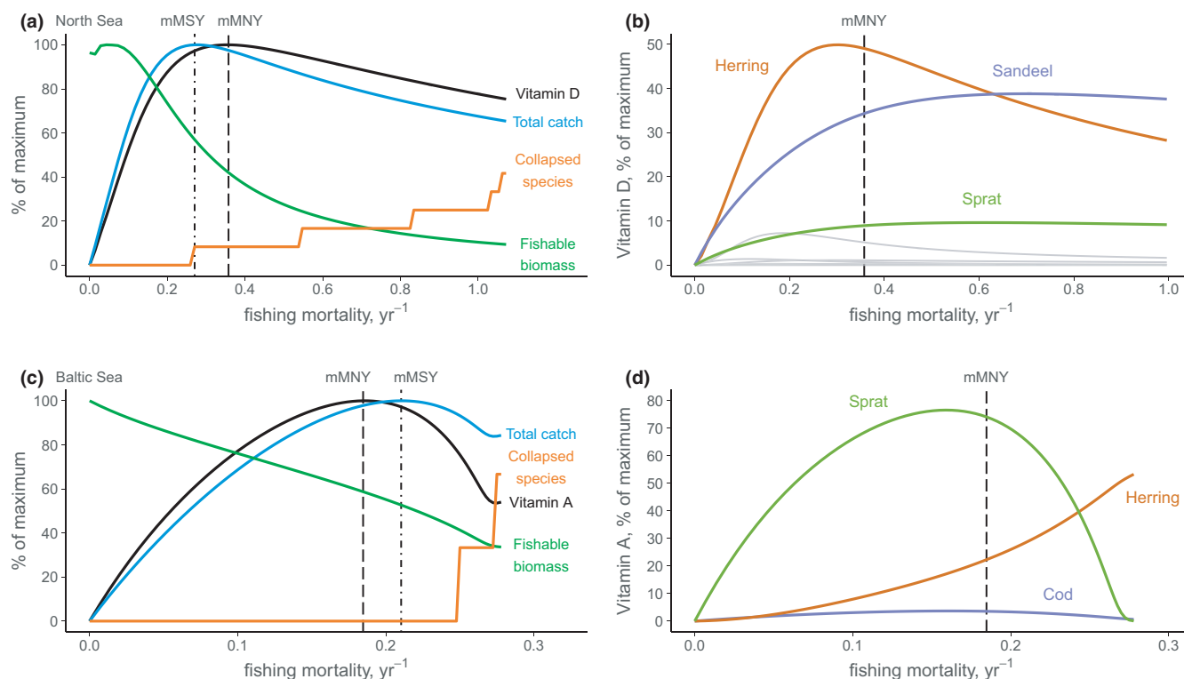
FIGURE 2 Nutrient yield curves in North Sea and Baltic Sea fisheries. (a) In the North Sea, maximum vitamin D yield occurred at fishing mortality above F_{mMSY} , owing to (b) high contribution of sandeel (purple), herring (orange) and sprat (green) to vitamin D yields. The remaining nine species (grey) contributed <5% of the maximum vitamin D yield owing to their low productivity and/or low vitamin D concentration. (c) In the Baltic Sea, maximum vitamin A yield occurred at fishing mortality below F_{mMSY} , owing to relatively high contribution of (d) sprat and herring to selenium yields. Fishing mortality is total catch/total biomass
